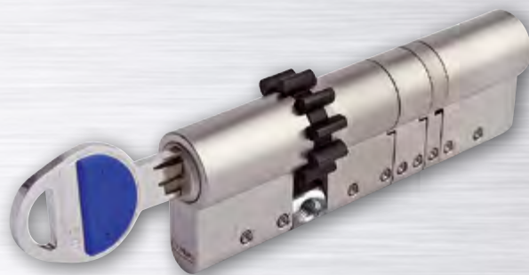
DOUBLE CYLINDER TOKOZ TECH WITH SPROCKET (10 TEETH)
