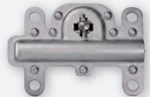
special eyelet for opening from the inside
