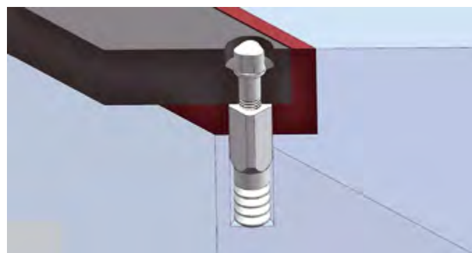
Security screw + chemical anchor housing
